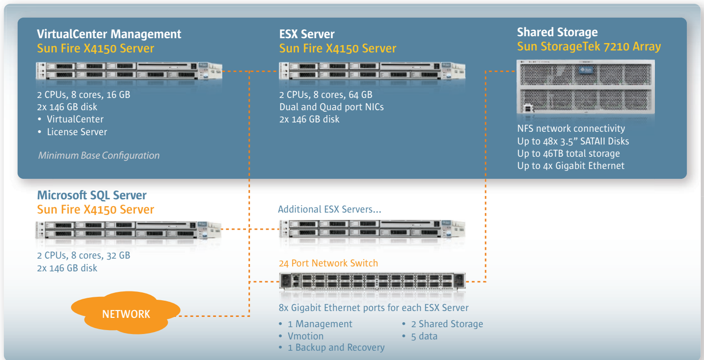
Sun Solution for Virtualization with VMware ESX — Typical Medium Configuration
